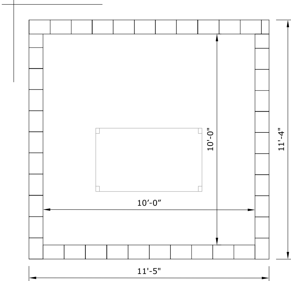
PLAN
